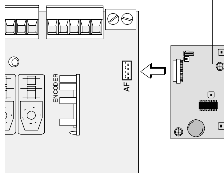
SCHEDA RADIOFREQUENZA "AF" "AF" RADIO FREQUENCY BOARD CARTE FREQUENCE RADIO "AF" RADIOFREQUENZKARTE «AF» TARJETA RADIOFRECUENCIA AF
