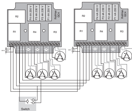
Fig. 3. GC4 block connection diagram
